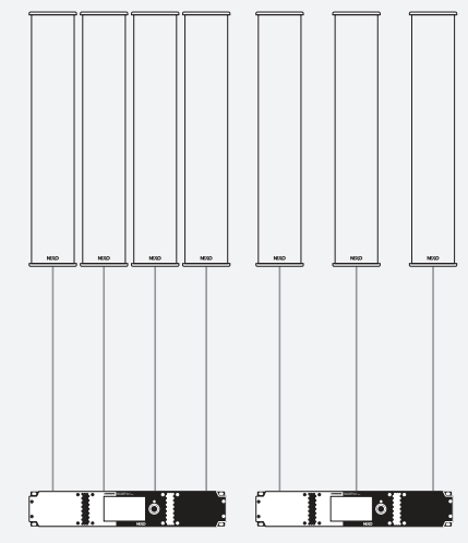
1 x ID84 per channel, powered by NXAMP4X1MK2
